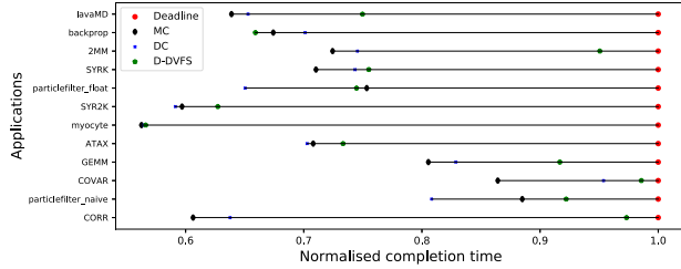
Fig. 8: Normalised application completion time compared to deadline
